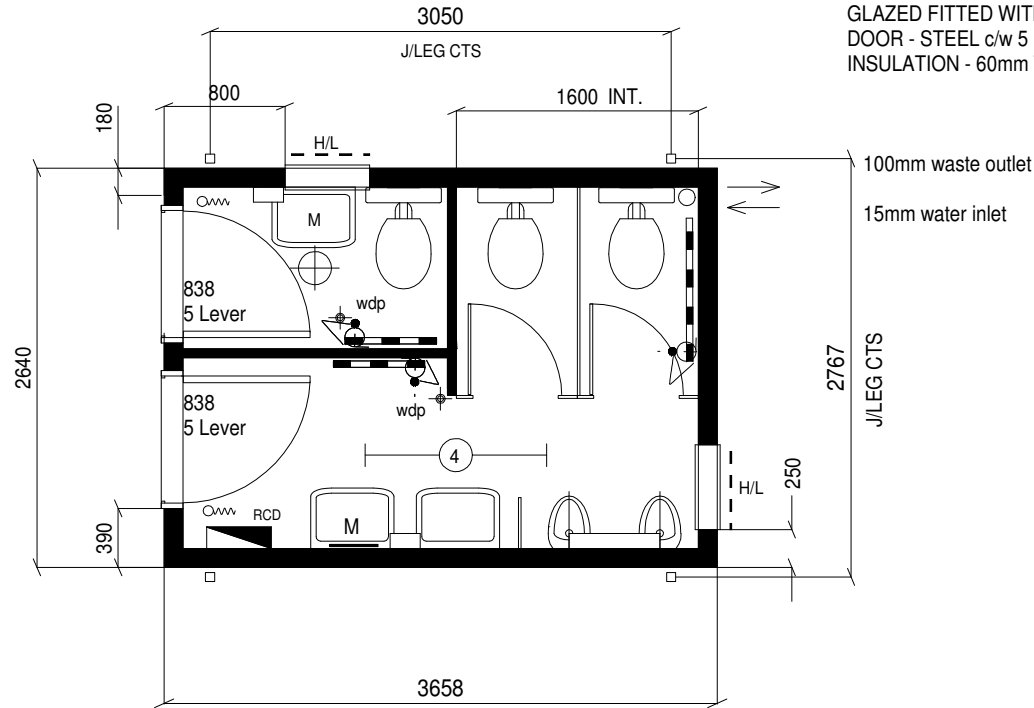
PLAN LAYOUT
